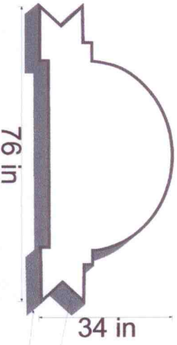
Internally Illuminated Cabinet with Digital Printed Image applied to plexiglas face
