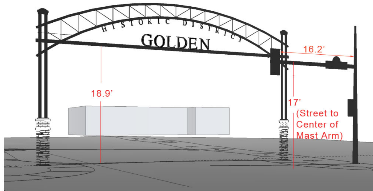
From Crosswalk: Arch Raised 2.5 Feet, Lowered Traffic Arm
